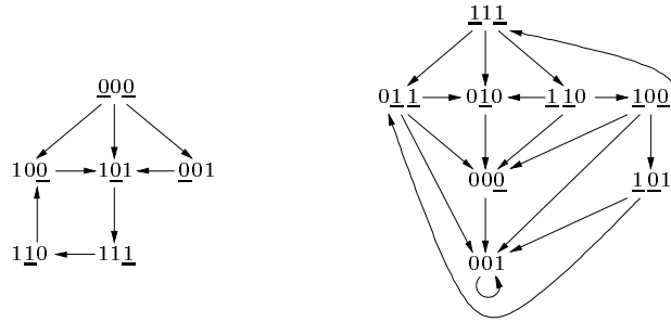
Fig. 3. Sample G_a(b) graphs for circuit of Fig. 1
