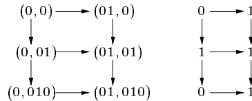
Fig. 5. Graph D(01, 010) with labels
